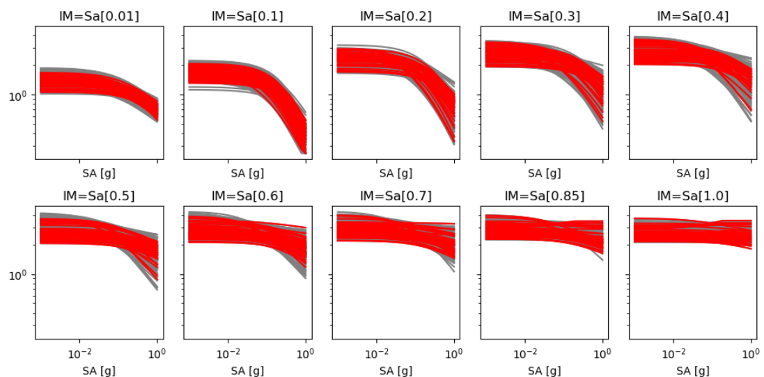
Figure 4-5 Median site amplification as a function of reference spectral acceleration per spectral component for all zones. The grey curves represent the 160 zones of the GMM-V&S, while the red curves represent the 81 new zones for KEM-19B. The curves are produced for an earthquake of magnitude 4.5 at distance of 15 km, to be able to compare to Figure 8.8 in Bommer et al. (2021).
